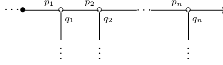
FIGURE 2. Path in splice diagram at infinity
